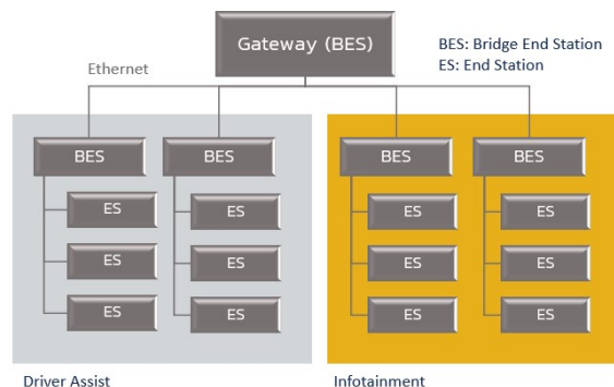
Figure 2. Multi-port Ethernet Domain Gateway.
